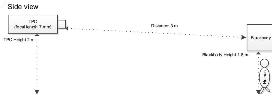
Figure 4-1 Installation (side view)
