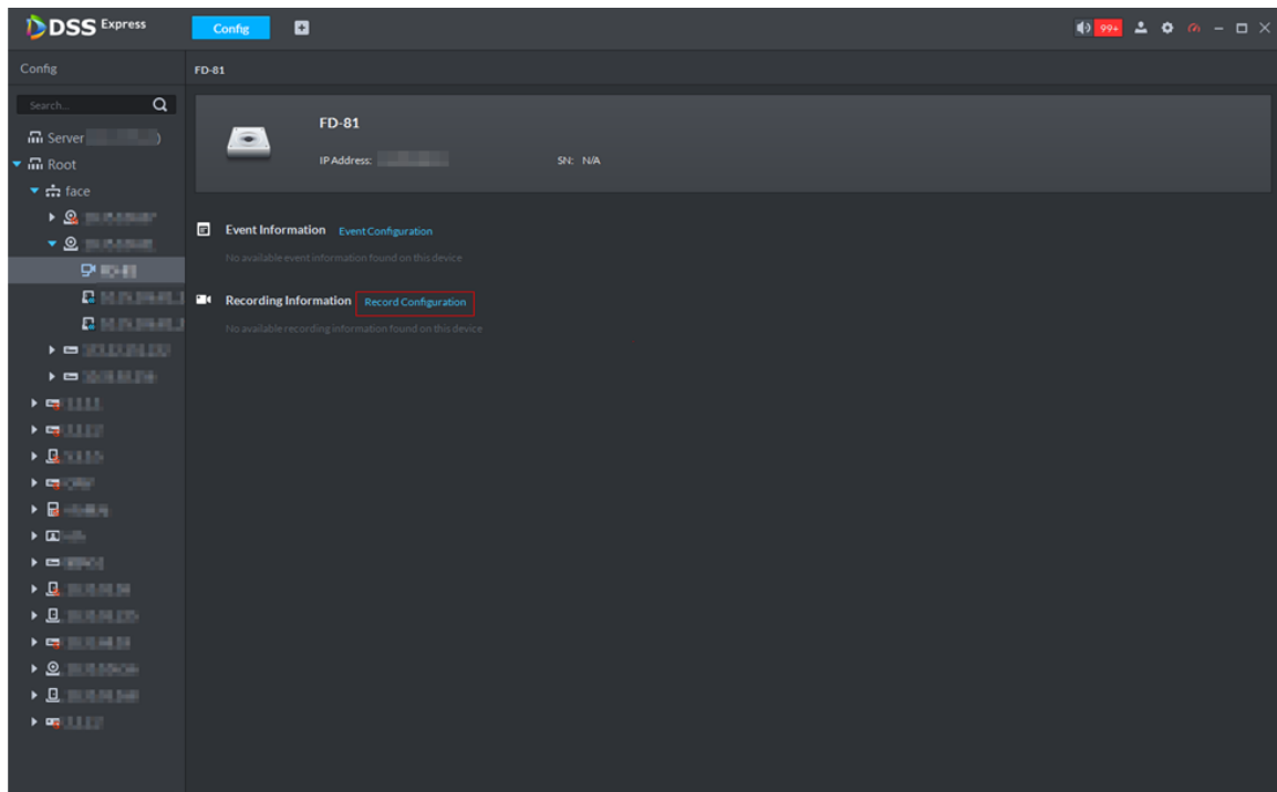
Figure 5-34 Record
