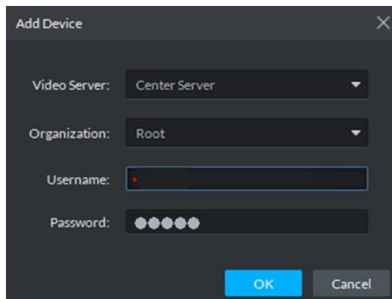
Figure 5-26 Add Device
