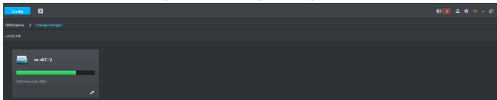
Figure 5-29 Storage manager
