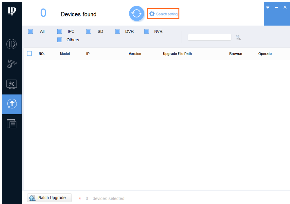
Figure 5-4 Update
