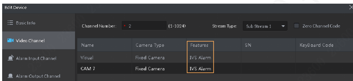
Figure 5-28 Edit device
