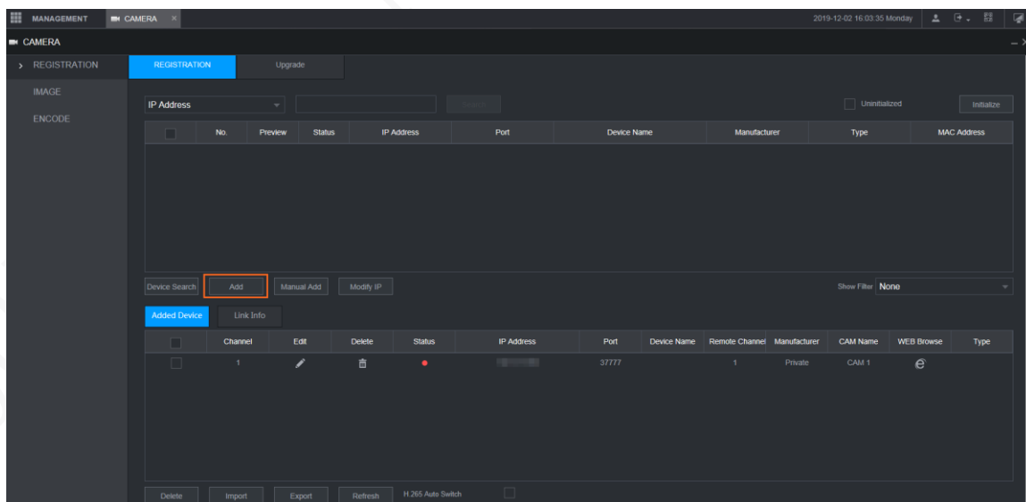
Figure 5-51 Camera (1)
