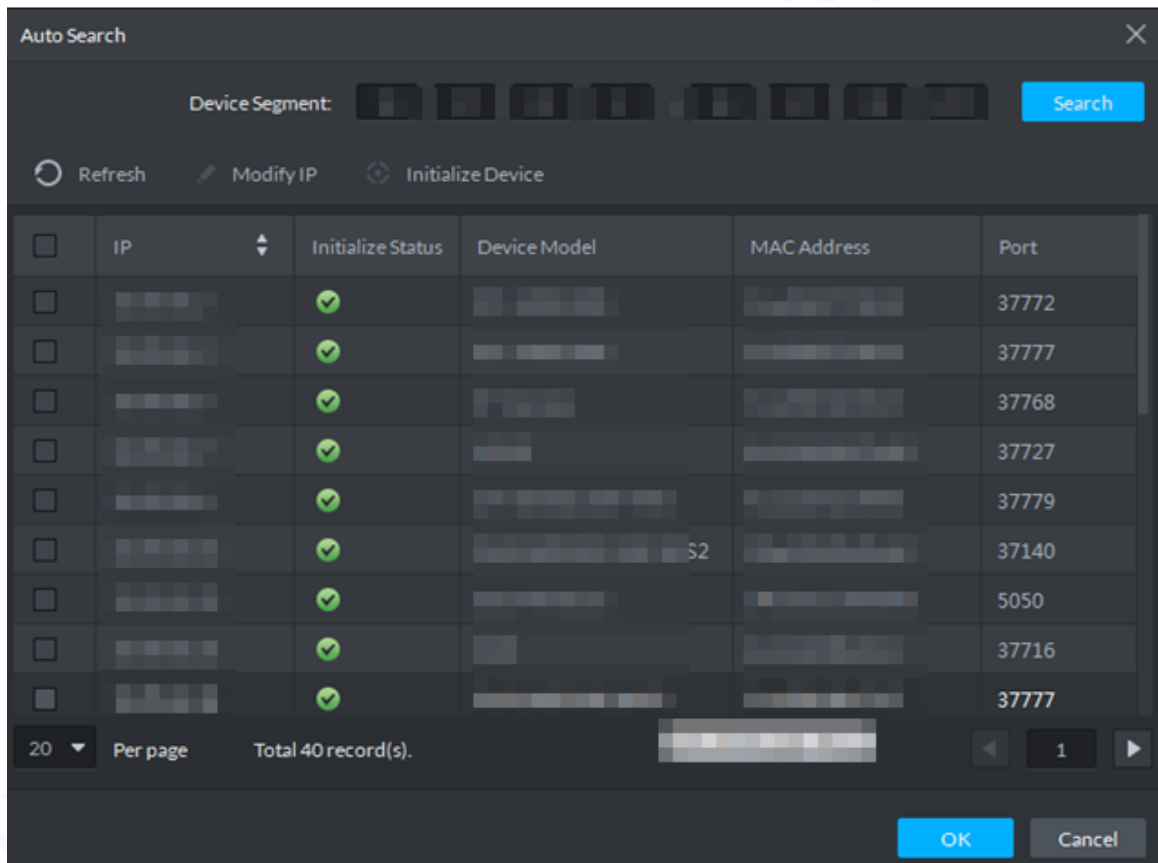
Figure 5-36 Auto search
