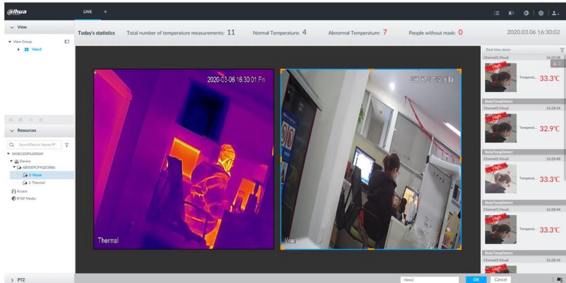
Figure 6-17 Live view
