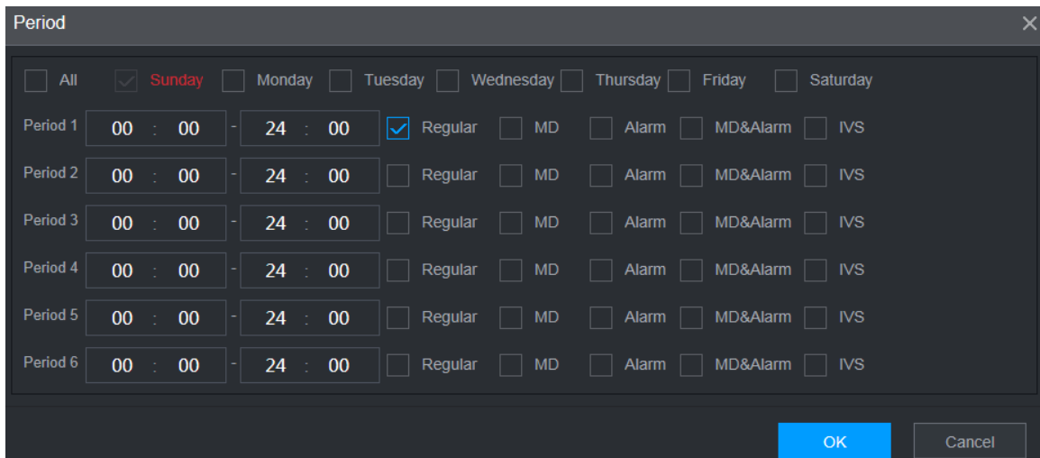
Figure 5-55 Period
