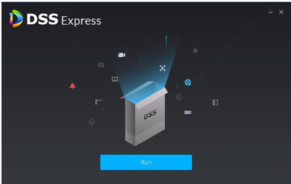
Figure 5-12 Installation completed
