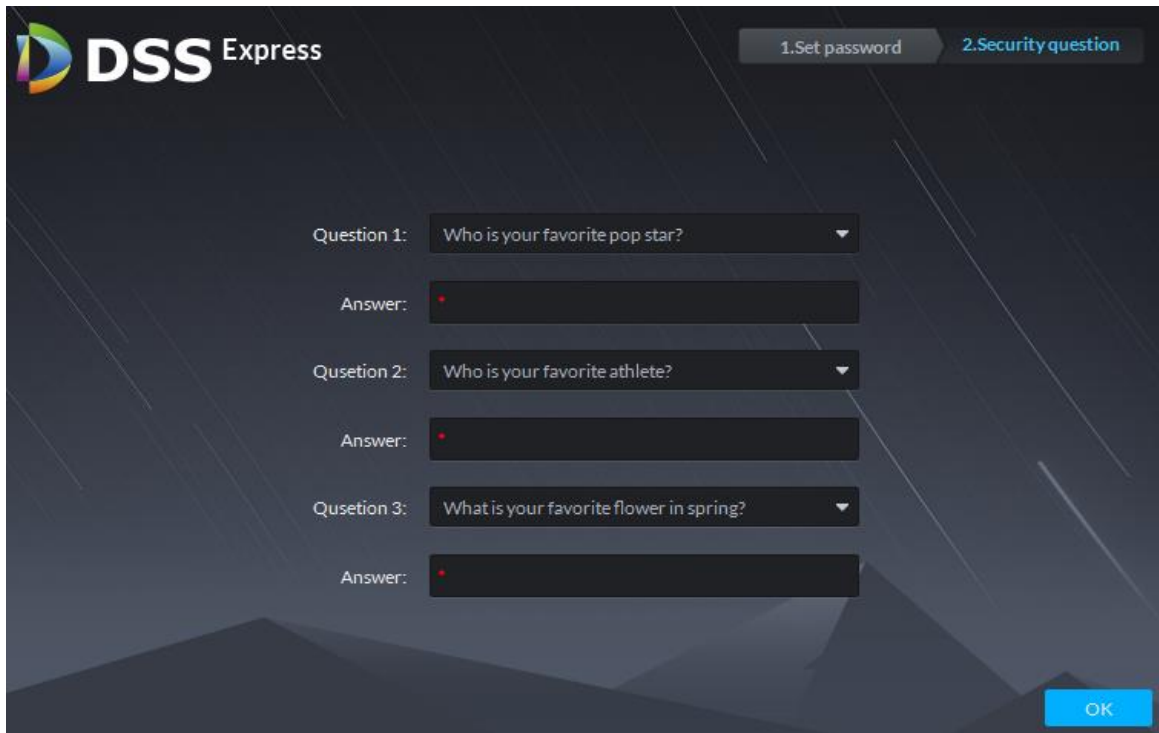
Figure 5-19 Security question
