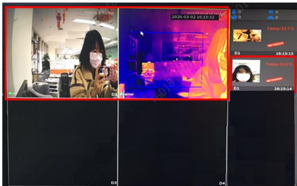
Figure 6-18 Live view
