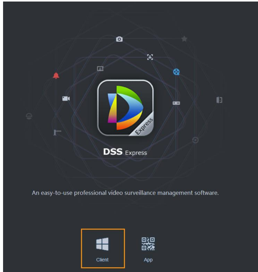
Figure 5-13 Download client
