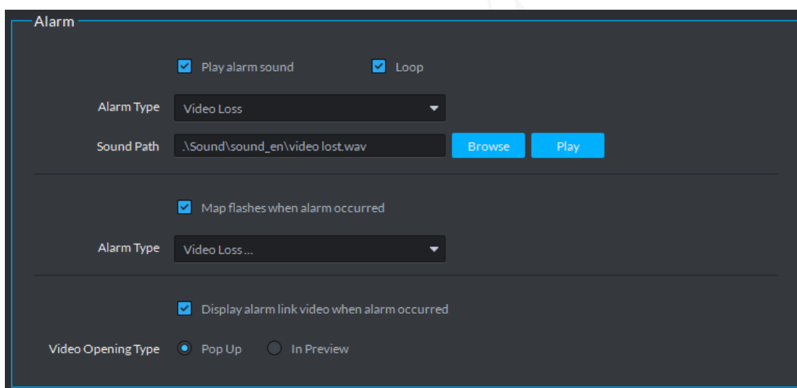
Figure 6-9 Alarm
