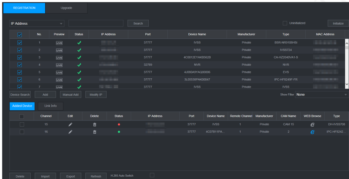
Figure 5-52 Camera (2)
