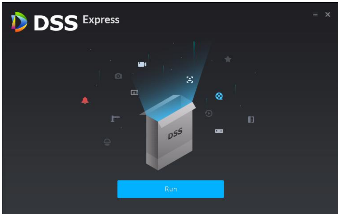
Figure 5-16 Installation completed
