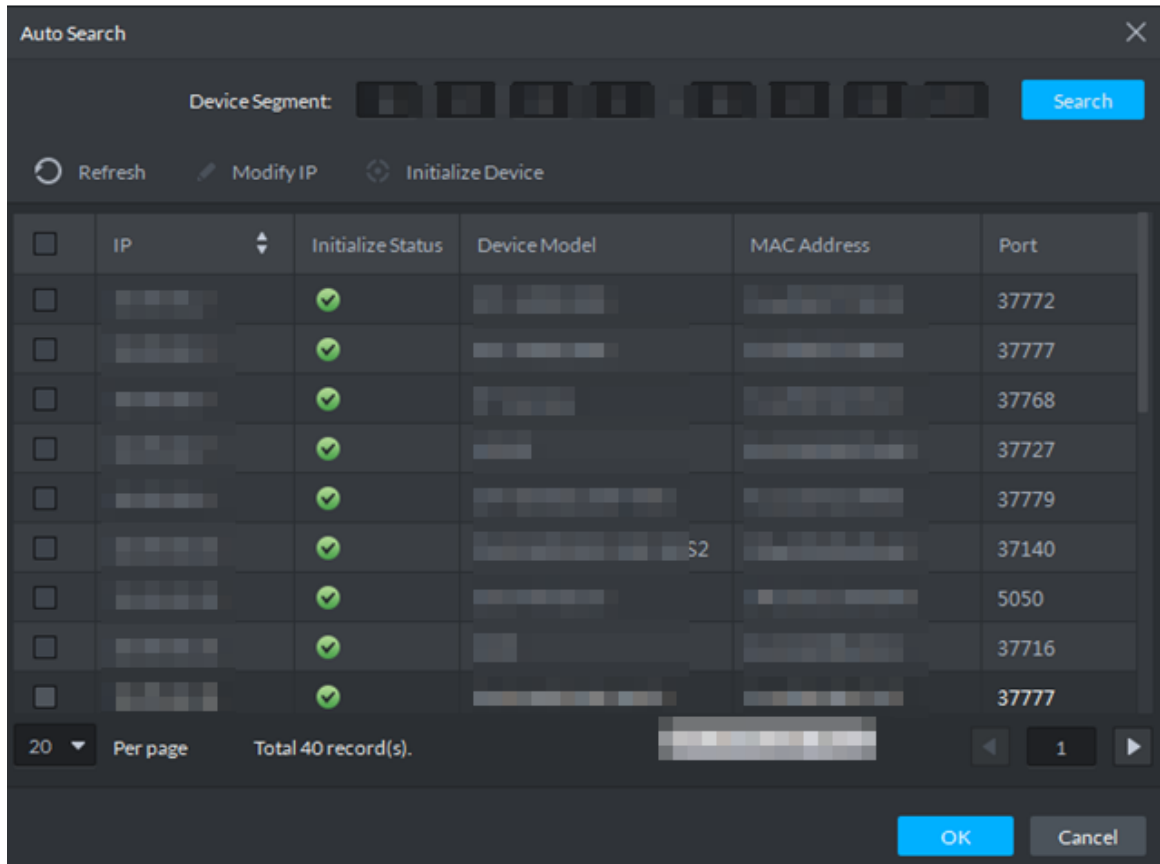
Figure 5-25 Auto search
