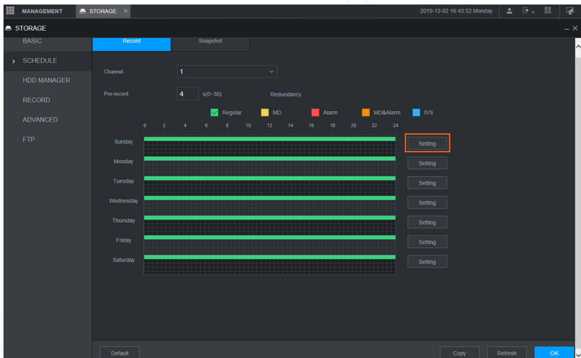
Figure 5-54 Record
