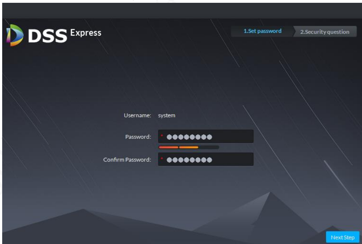
Figure 5-18 Set password
