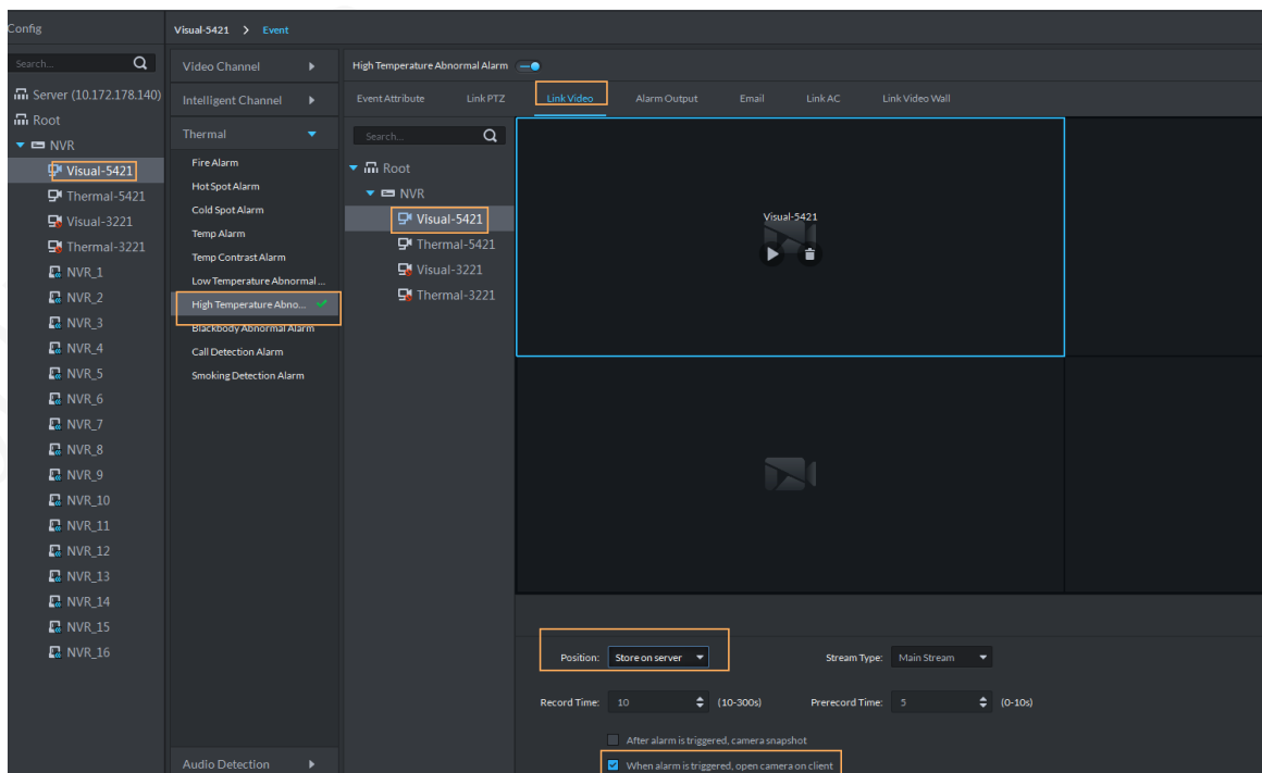
Figure 6-8 Link video
