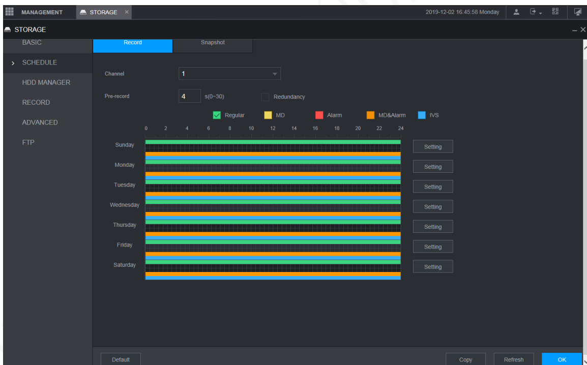
Figure 5-56 Record plan
