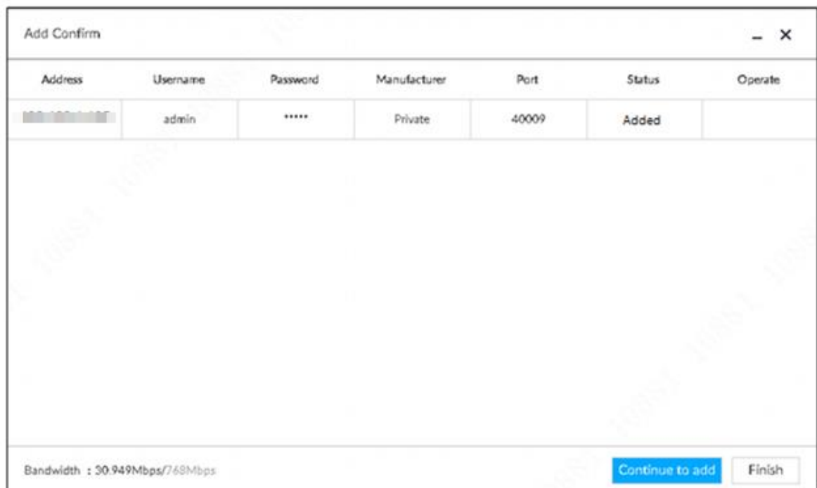
Figure 5-49 Confirm
