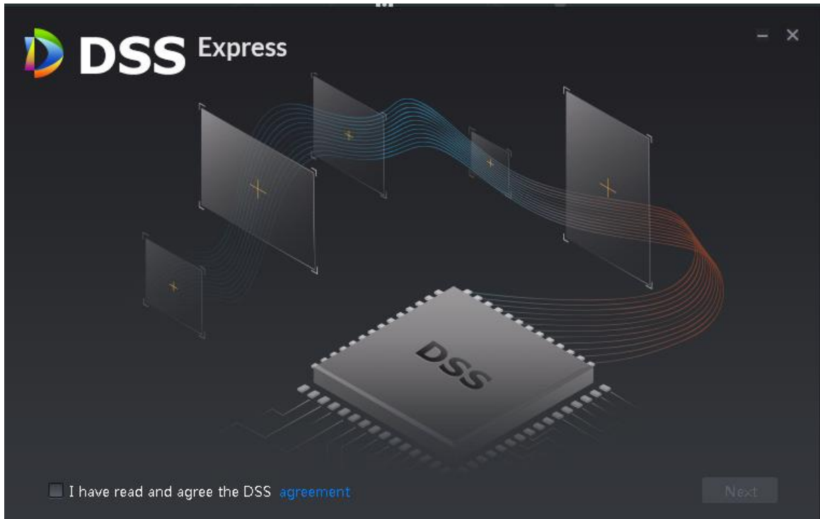
Figure 5-14 Confirm agreement
