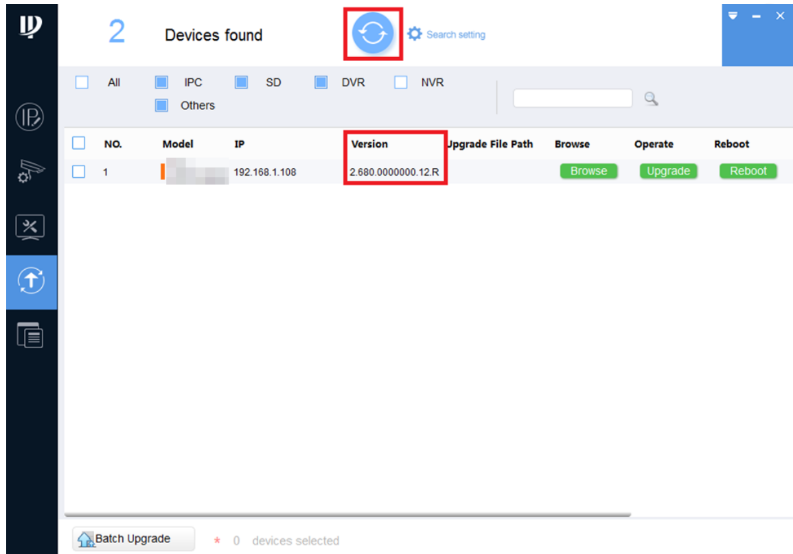
Figure 5-10 Confirm version
