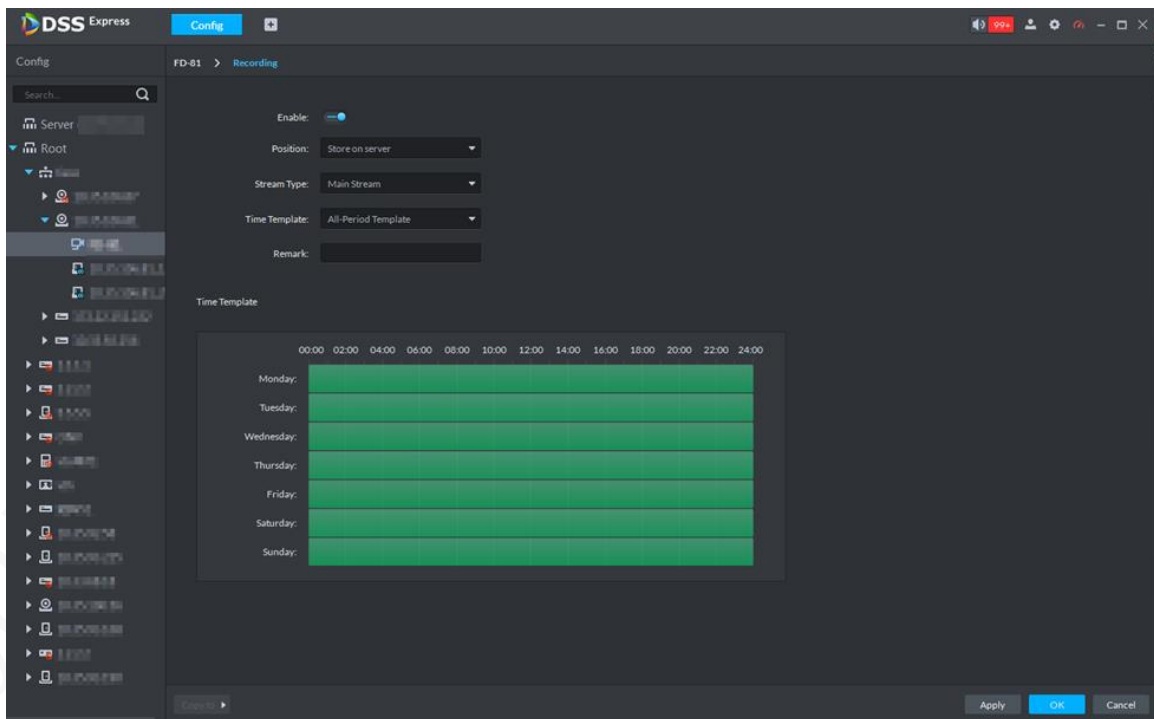
Figure 5-34 Record
