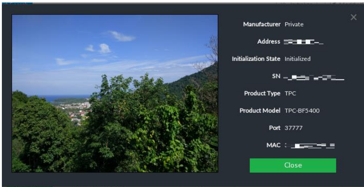
Figure 5-41 Live view
