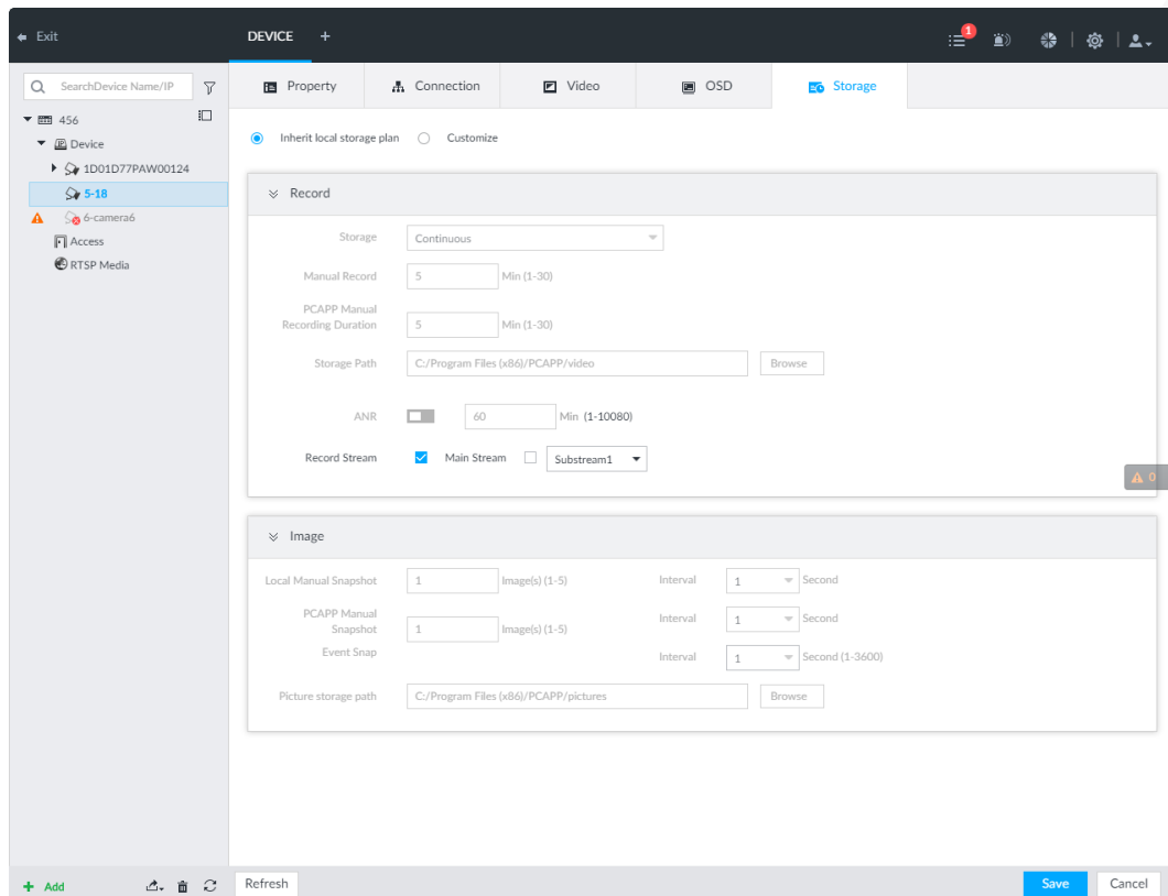
Figure 5-50 Storage
